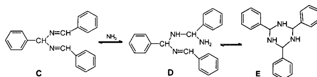
Scheme 3. Hydrobenzamide (C) in equilibrium with NH 3 , leading to compound D, and possibly E
