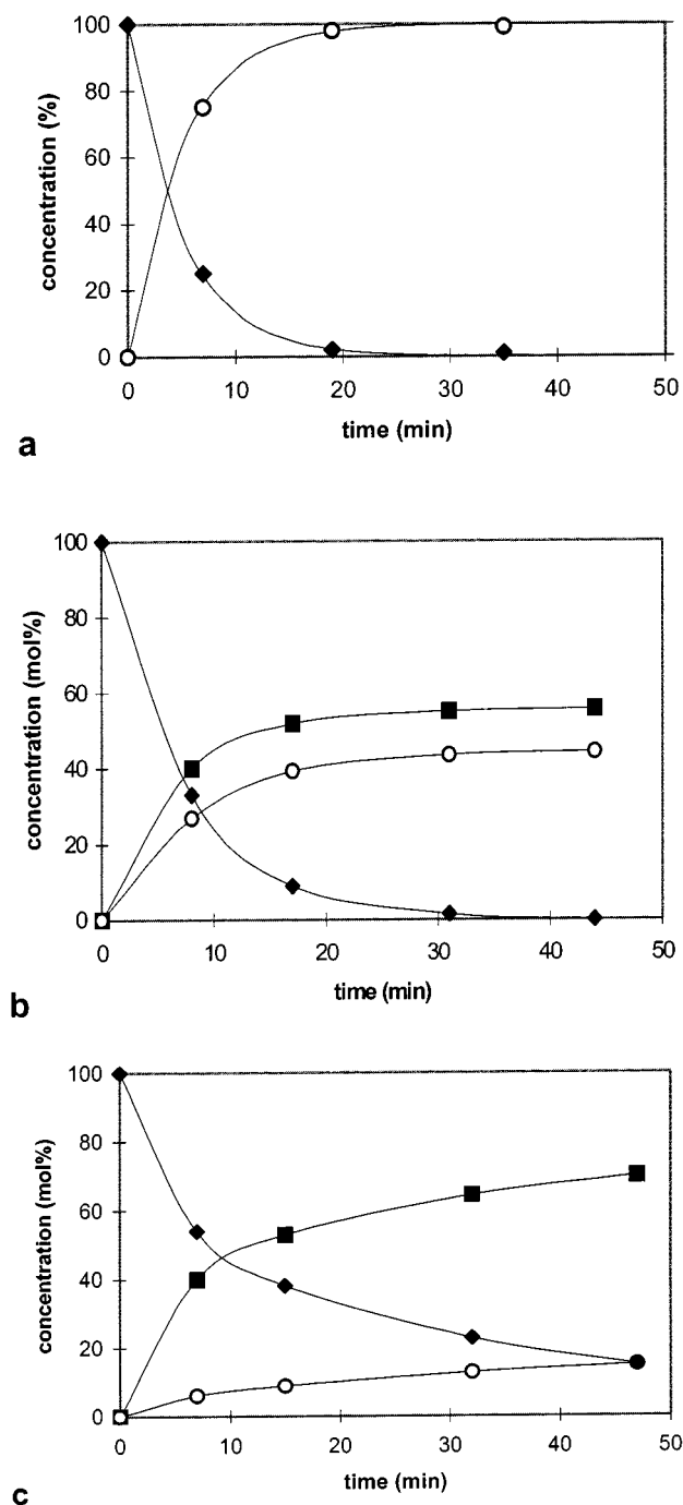
Figure 7. Hydrogenation of dibenzylimine in the presence of (a) 0 M \text{NH}_3 , (b) 1 M \text{NH}_3 , and (c) 4 M \text{NH}_3 ; Benzylamine (■), dibenzylamine (○), and dibenzylimine (◆); 80 mL of \text{NH}_3/\text{MeOH} , 17 mg of Pd/SX1GNS150, 0.9 g of dibenzylimine, 90 °C and 40 bar \text{H}_2
