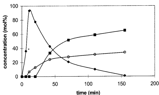
Figure 5. Concentrations of benzylamine (■), dibenzylamine (○), and dibenzylimine (◆) during the reductive amination of benzaldehyde; 80 mL of 2 M NH 3 /MeOH, 17 mg Pd/SX1GNS150, 1 g of benzaldehyde, 90 °C and 40 bar H 2 . *At this point, the mass balance was < 100%, most probably due to the formation of hydrobenzamide when the sample was cooled down. This compound was not analyzed, but could be precipitated on the catalyst
