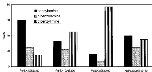
Figure 8. Composition of the reaction mixture after 2 h in the reductive amination of benzaldehyde with ammonia over 5% Pd/C catalysts, reduced at different temperatures; 80 mL of 2 M \text{NH}_3/\text{MeOH} , 17 mg of catalyst, 1 g of benzaldehyde, 90 °C and 40 bar \text{H}_2
