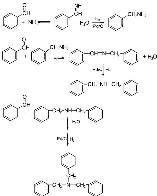
Scheme 1. Overall steps in the reductive amination of benzaldehyde
