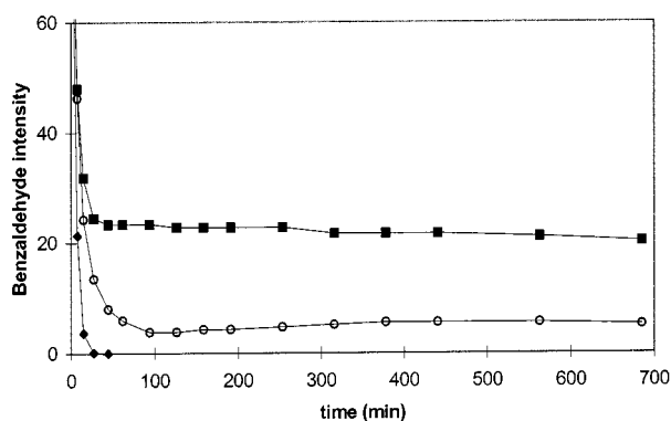
Figure 4. Relative intensity of the benzaldehyde peak ( \delta = 9.9 ) vs. time during the reaction with benzylamine to dibenzylimine in [D_4]MeOH (25 °C) at different benzaldehyde/benzylamine/ D_2O ratios: (○) 1:1:1:0; (◆) 1:2:1:0; (■) 1:1:1:2.6
