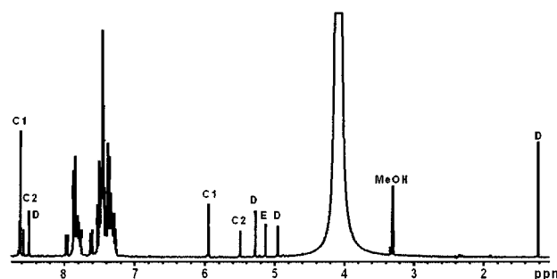
Figure 2. 1 H NMR spectrum of a mixture of benzaldehyde and NH 3 in [D 4 ]MeOH. C1 and C2 indicate resonances of the different isomers of hydrobenzamide (C, Scheme 3); D and E mark the resonances of compound D and E (Scheme 3), respectively
