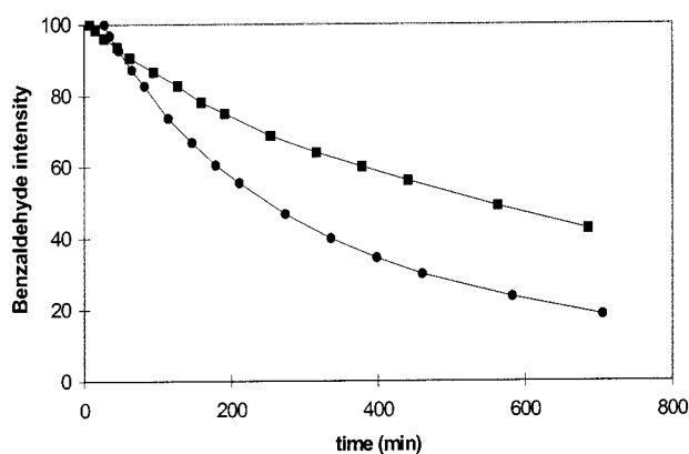
Figure 3. Relative intensity of benzaldehyde peak ( \delta = 9.9 ) vs. time during the reaction with ammonia to hydrobenzamide in [D_4]MeOH at (a) 25 °C and different benzaldehyde/ NH_3 / D_2O ratios: (◆) 1:1:0; (■) 1:2:0; (□) 1:2:1.6; (●) 1:10:0; and (b) benzaldehyde/ NH_3 = 1:1 and different temperatures: (■) 25 °C and (●) 40 °C
