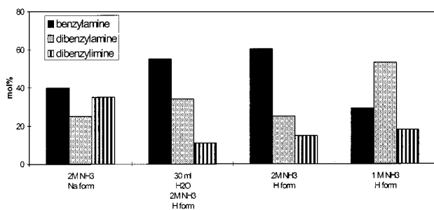
Figure 6. Composition of the reaction mixture after 2 h in the reductive amination of benzaldehyde with ammonia over 5% Pd/SX1GNS150. Effect of the cationic form of the catalyst, of addition of water and of NH 3 concentration; 80 mL solution, 17 mg of Pd/SX1GNS150, 1 g of benzaldehyde, 90 °C and 40 bar H 2
