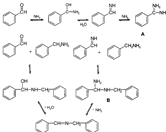
Scheme 2. Equilibria leading to benzylimine and dibenzylimine
