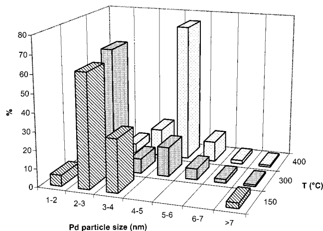
Figure 1. Pd particle size distribution of Pd/SX1GNS versus catalyst reduction temperature
